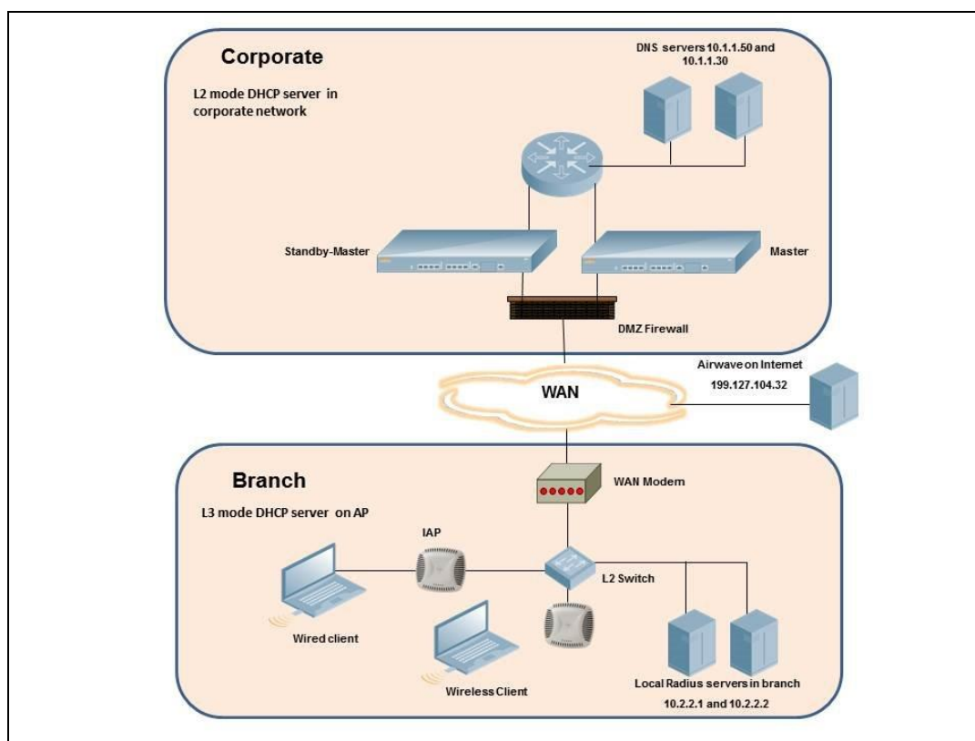
Figure 121 Scenario 2—IPSec: Single Datacenter with Multiple switches for Redundancy
